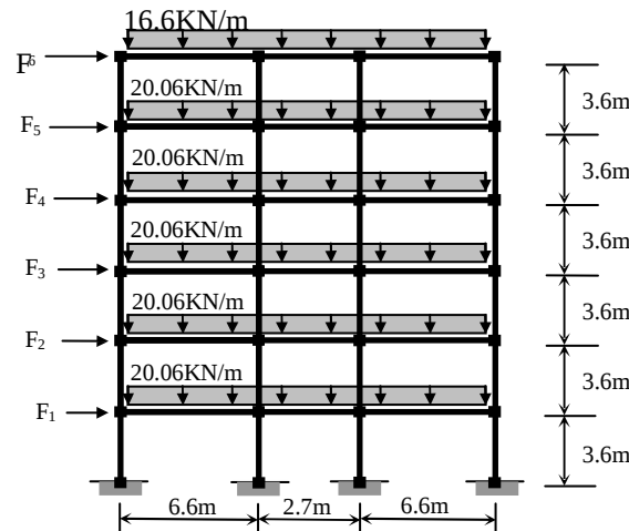
Figure 1 Three-bay and six-storey R.C. frame
