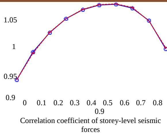
Figure 5 Changing of global seismic reliability index with the correlation coefficient of seismic forces
