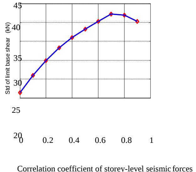
(b) Std of limit base shear
