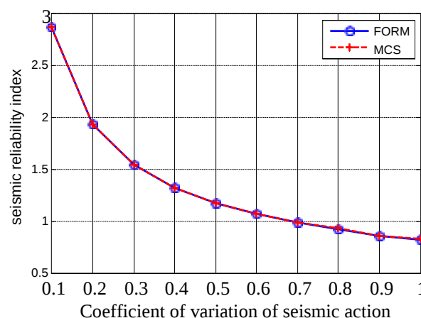
Figure 4 Changing of global seismic reliability index with the COV of seismic action
