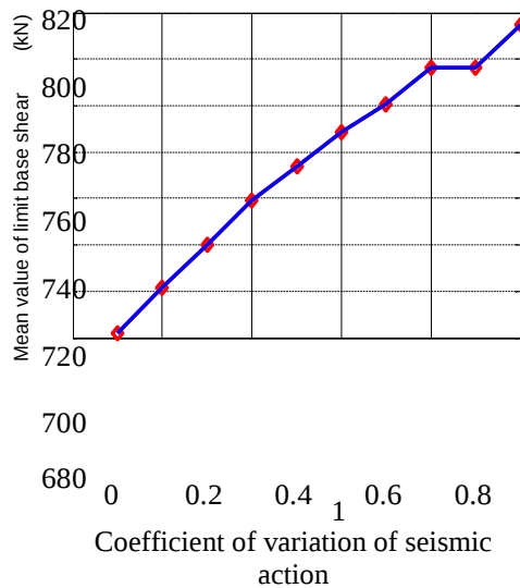
(a) Mean value of limit base shear
